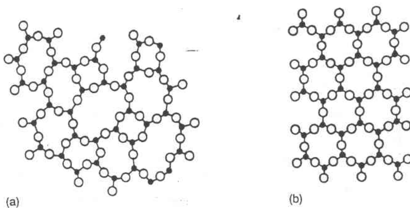
Fig. 2.3 (a) A two-dimensional representation of an amorphous, covalently bonded structure, in which one type of atom (•) is trigonally coordinated and another (o) is two-fold coordinated. A real example might be B_2O_3 . (b) The corresponding crystalline modification of the amorphous structure shown in (a).
